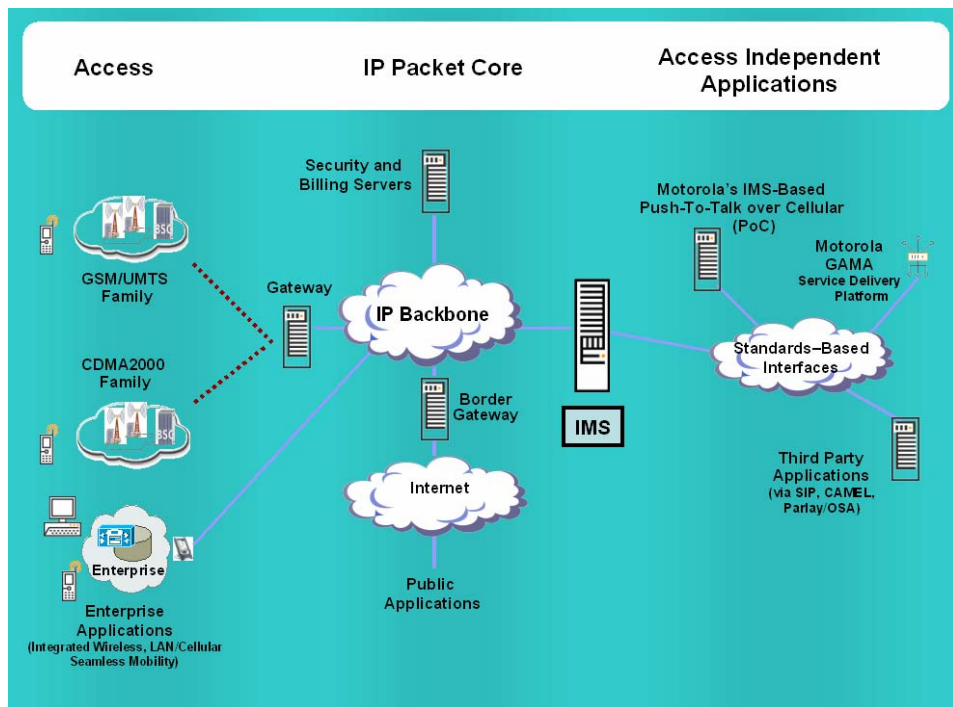
Figure 2— Motorola IMS Architecture
