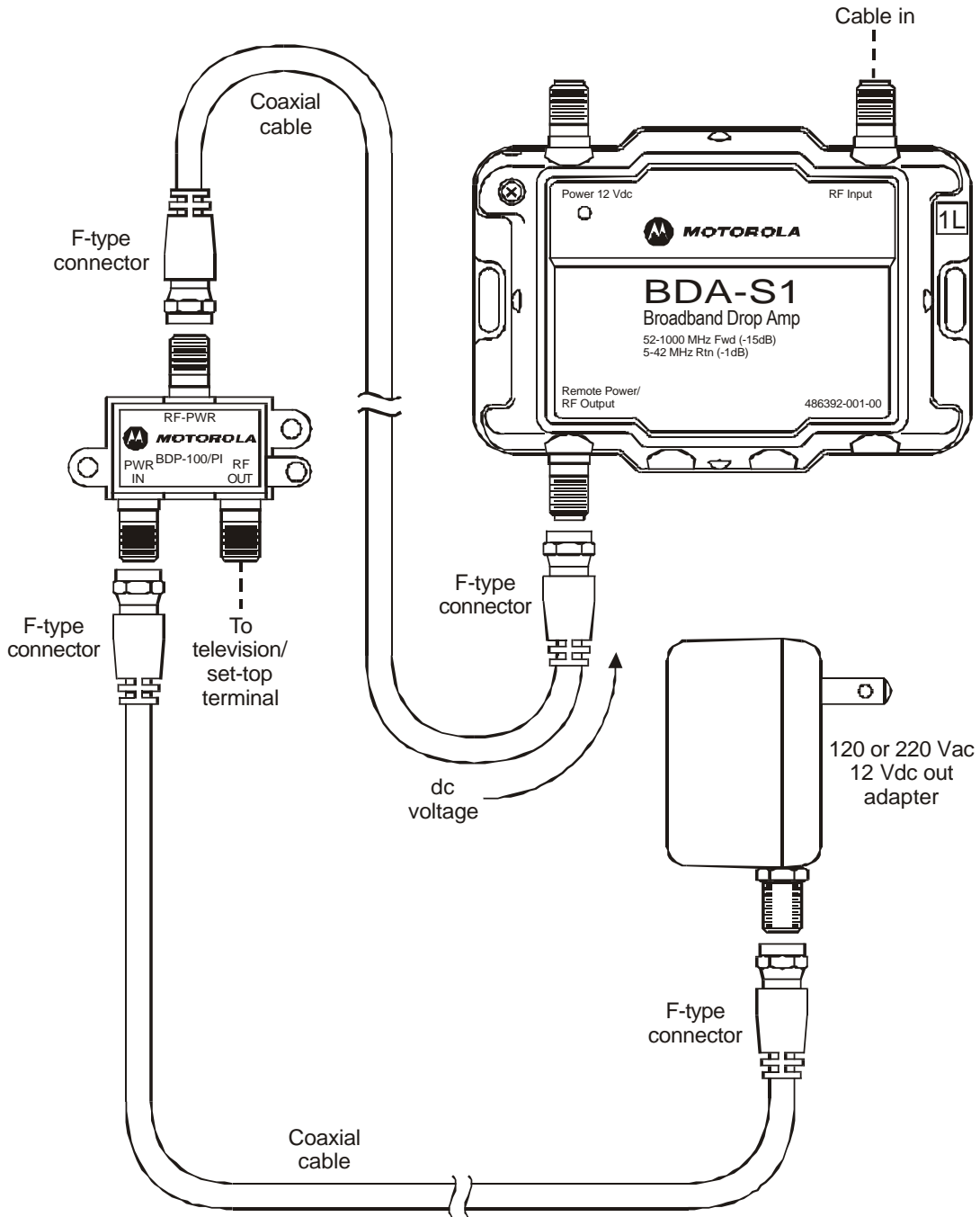
Figure 4 Remote-power installation
