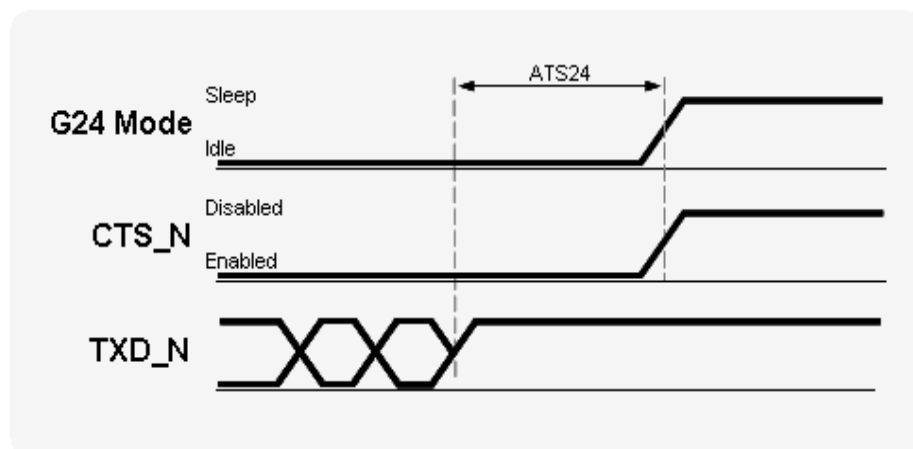
Figure 2-7: AT S24 Operation
