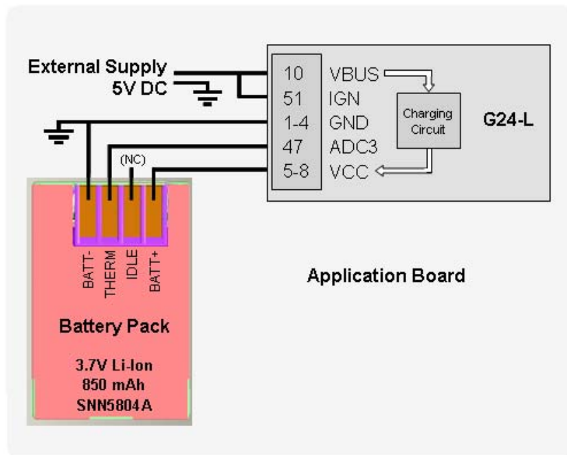
Figure 2-26: Battery and Charger Interface Connectivity
