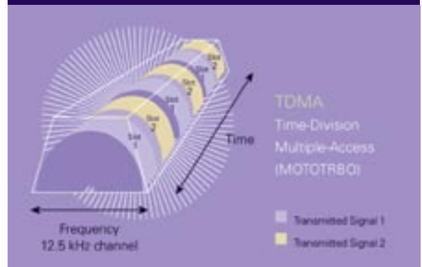
Increased Capacity Within Existing 12.5 kHz Repeater Channels
